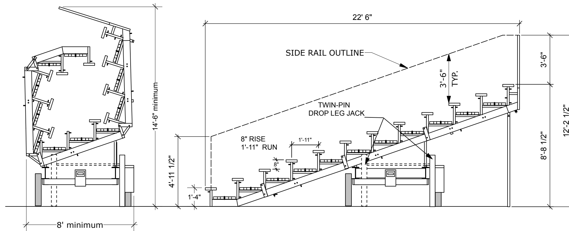
② ELEVATION (guardrails removed) Scale: 1/4" = 1'-0"
