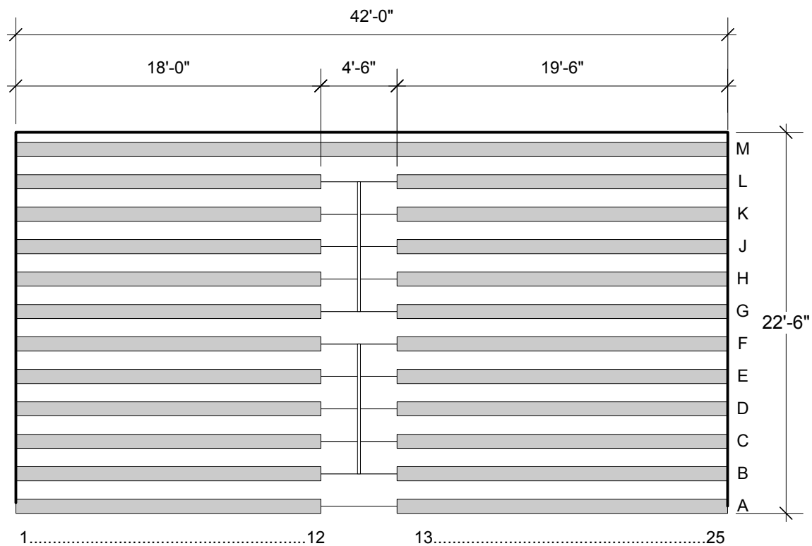
① PLAN VIEW (303 SEATS) Scale: 1/8" = 1'-0"
